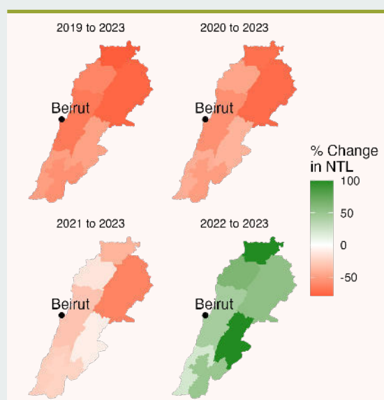
FIGURE 4 • Changes in NTL at the First Administrative (i.e., Governorate) Level
